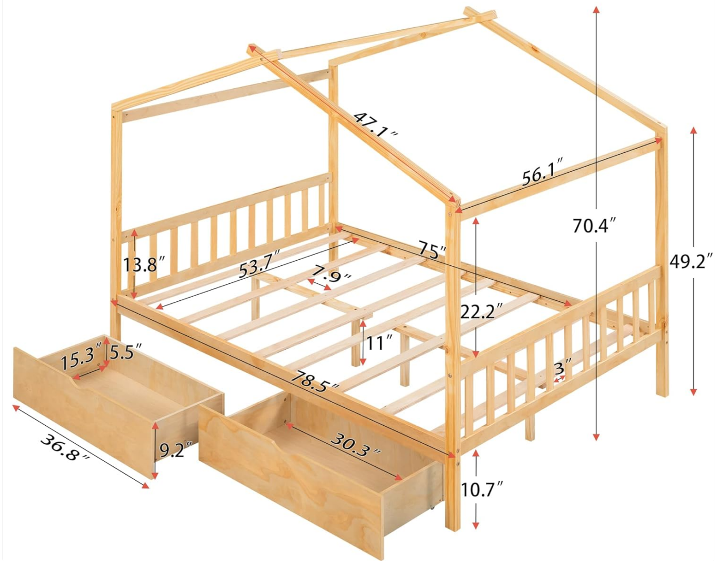
Figure 2.1: Dimensional diagram of the assembled bed frame.
