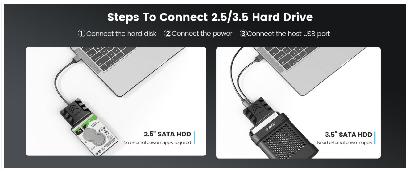
Image: A 2.5-inch SATA hard drive connected to the adapter. No external power is required for 2.5-inch drives.
