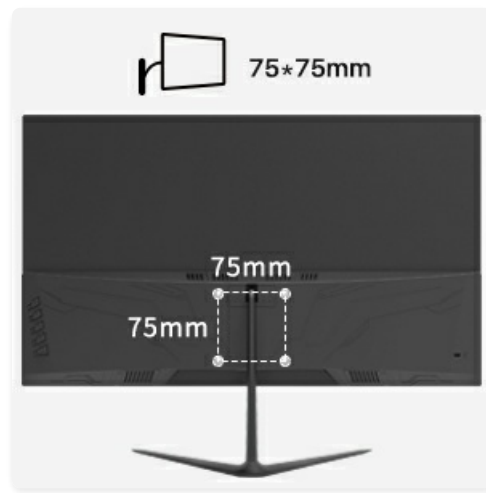
Image 3.2: VESA mounting pattern on the back of the monitor.
