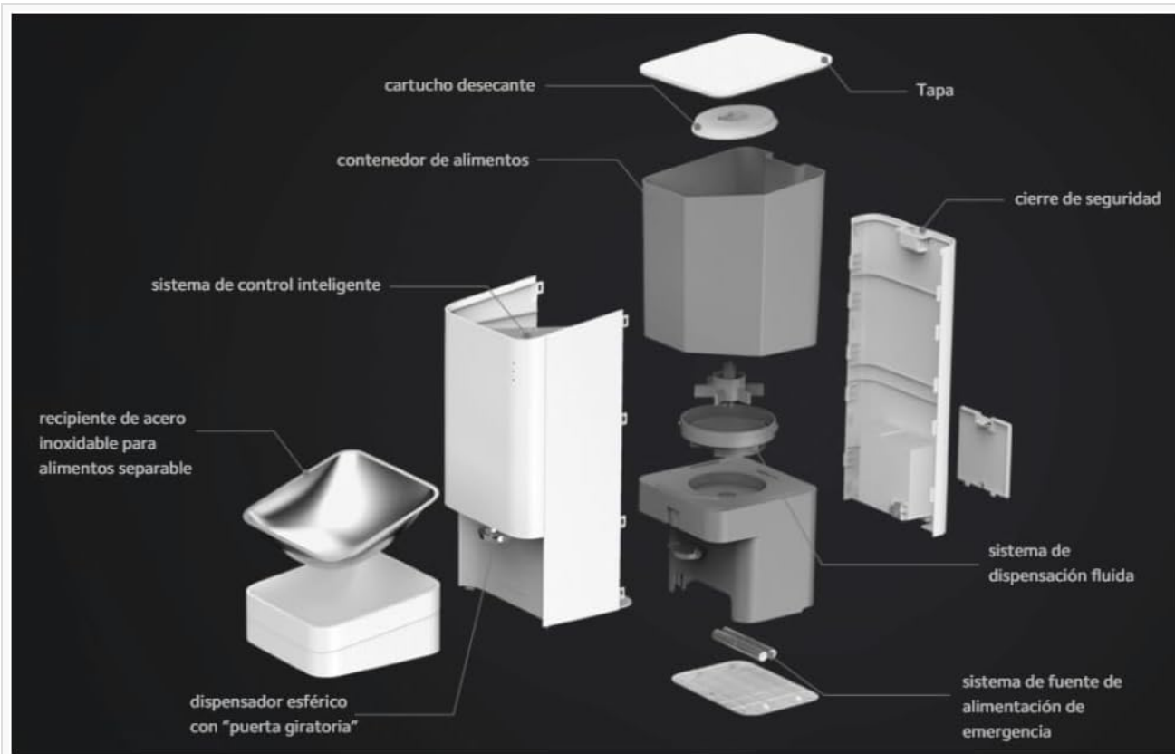
Figure 2: Exploded view of the feeder's components. This diagram illustrates the main parts including the lid, desiccant cartridge, food container, smart control system, food-grade stainless steel bowl, emergency power supply system (battery compartment), fluid dispensing system, and security lock.
