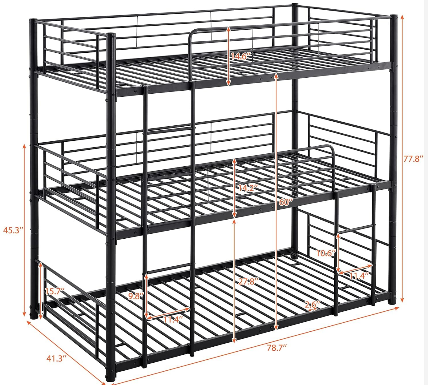
Figure 8.1: Detailed dimensions of the Moimhear Triple Twin Bunk Bed.
