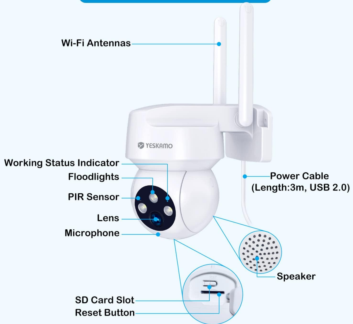
Image: Labeled diagram of the YESKAMO AP55 camera, highlighting Wi-Fi Antennas, Working Status Indicator, Floodlights, PIR Sensor, Lens, Microphone, Power Cable, Speaker, SD Card Slot, and Reset Button.
