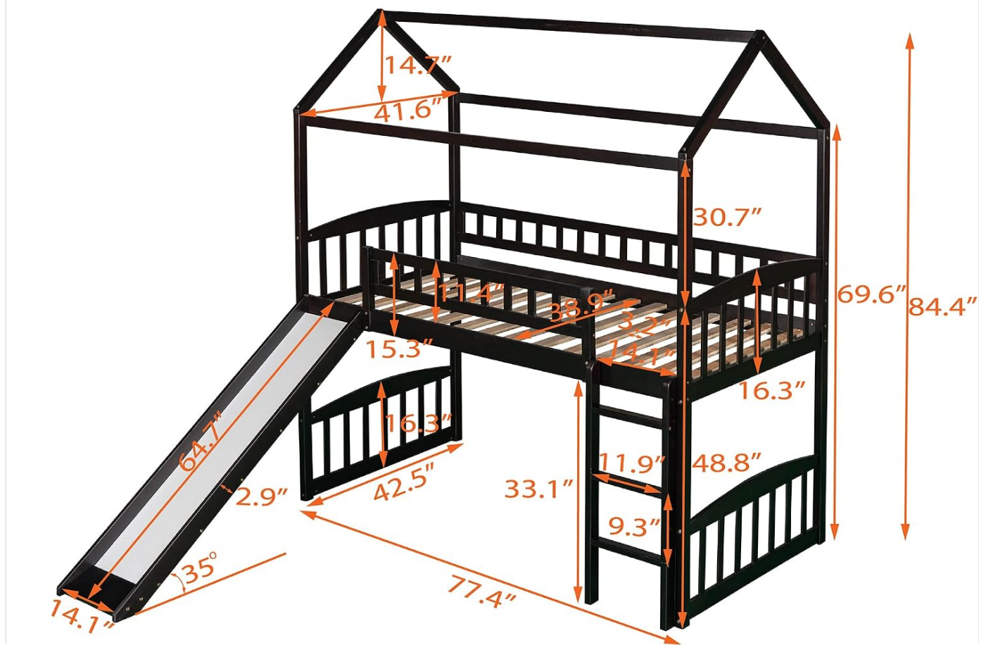
Image: A detailed diagram illustrating the overall dimensions of the Moimhear Twin Loft Bed, including length, width, height, and specific measurements for the slide and ladder.
