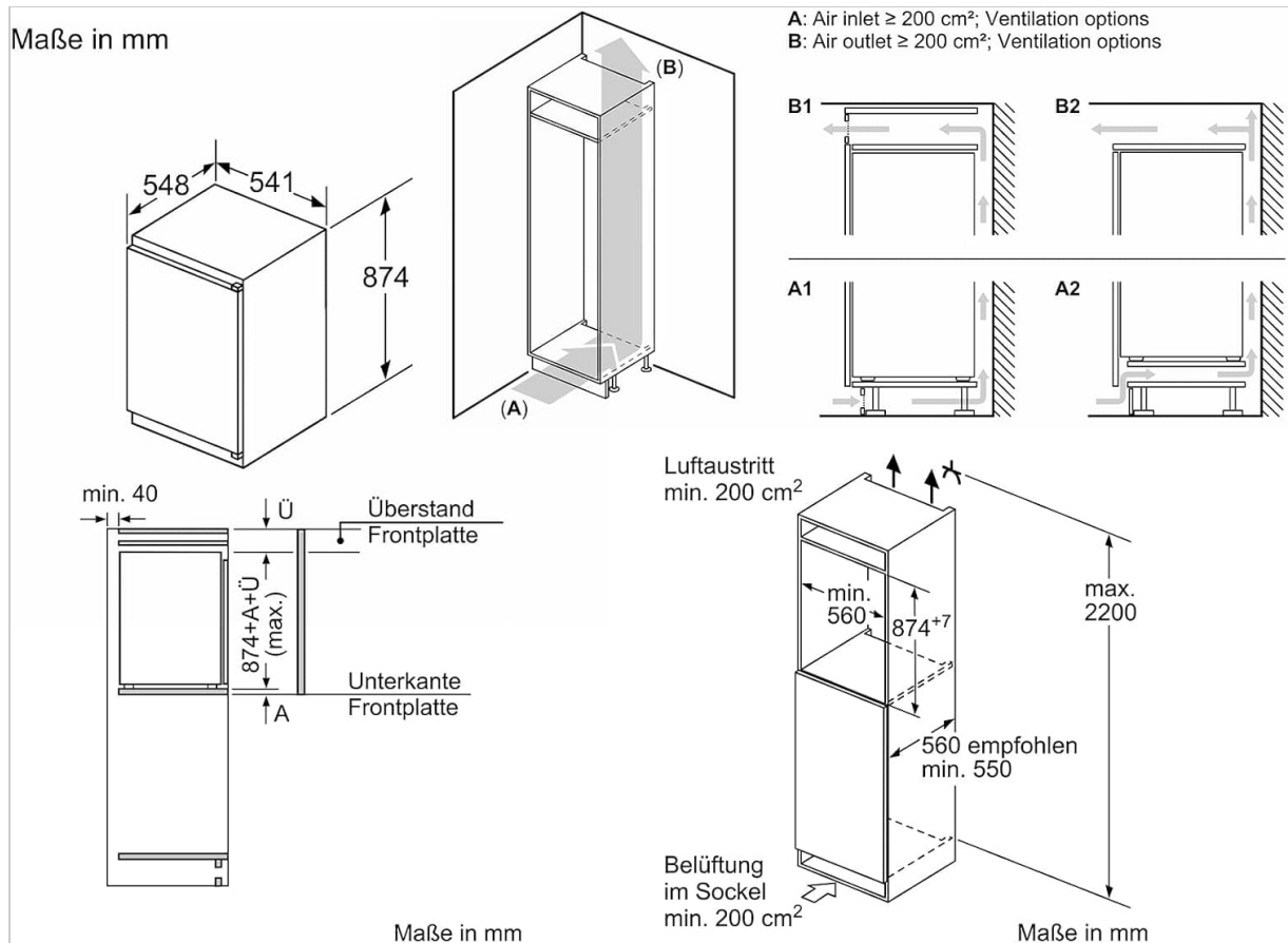
Figure 2: Installation diagram illustrating the refrigerator's dimensions and necessary ventilation spaces for proper air circulation. This includes measurements for depth, width, height, and recommended air inlet and outlet areas.
