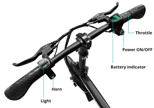
Figure 5.3: Handlebar controls for easy operation.
