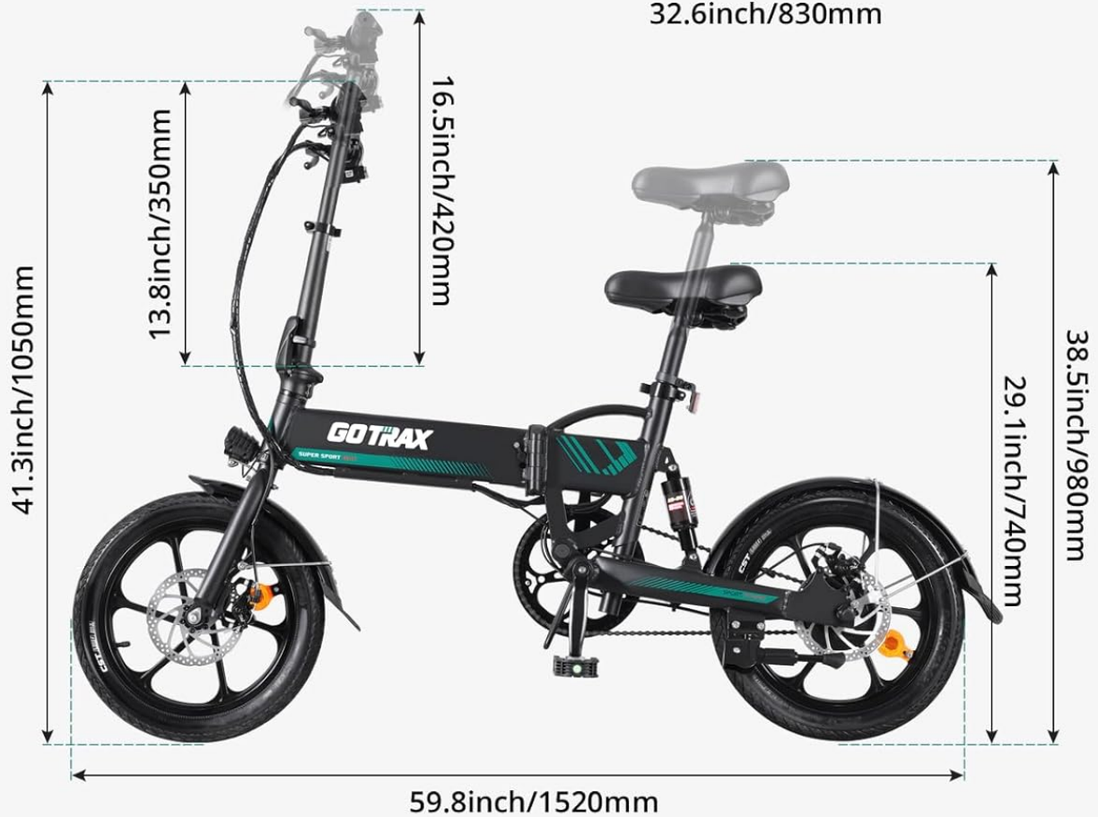
Figure 12.1: Detailed dimensions of the electric bike.
