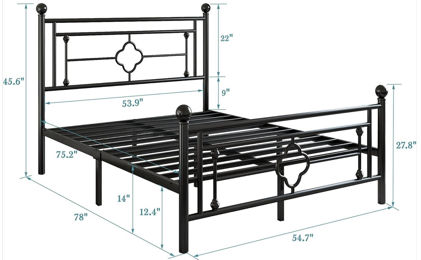
Image: Detailed diagram showing the dimensions of the HOOMIC Full Size Metal Platform Bed Frame, including length, width, height, and under-bed clearance.
