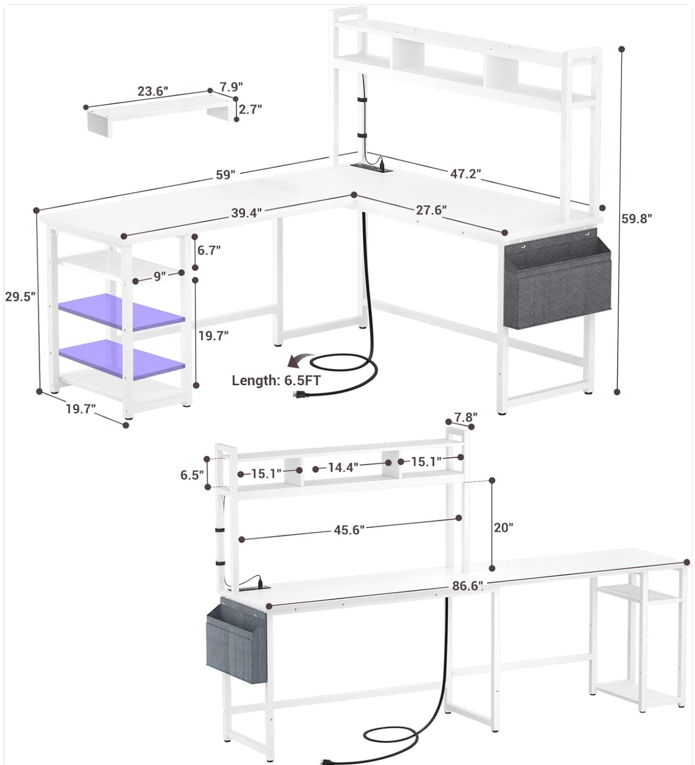
Figure 2: Detailed dimensions of the Aheaplus L Shaped Desk in both L-shaped and long table configurations, including shelf and hutch measurements.
