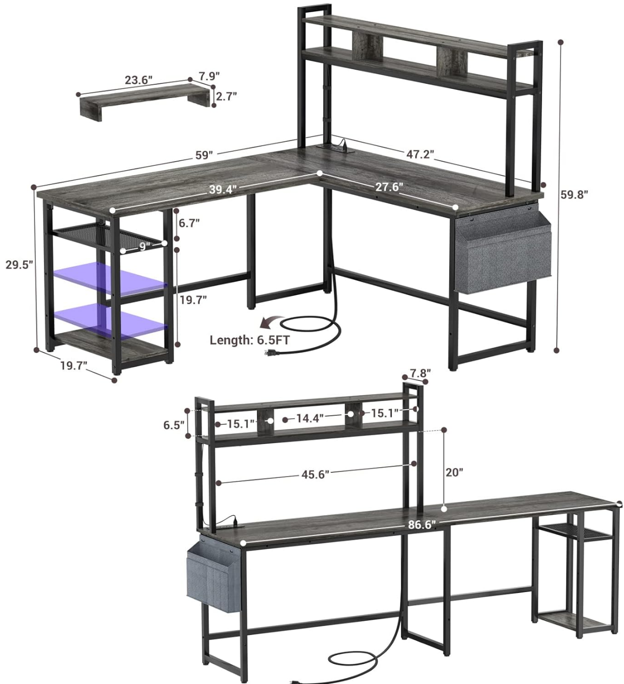
Figure 3.1: Detailed dimensions of the Aheaplus L Shaped Desk in both its L-shaped and straight configurations, providing measurements for planning your space and ensuring all components fit.
