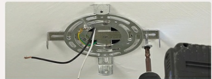
STEP 2 Fix the hanger on the ceiling.
