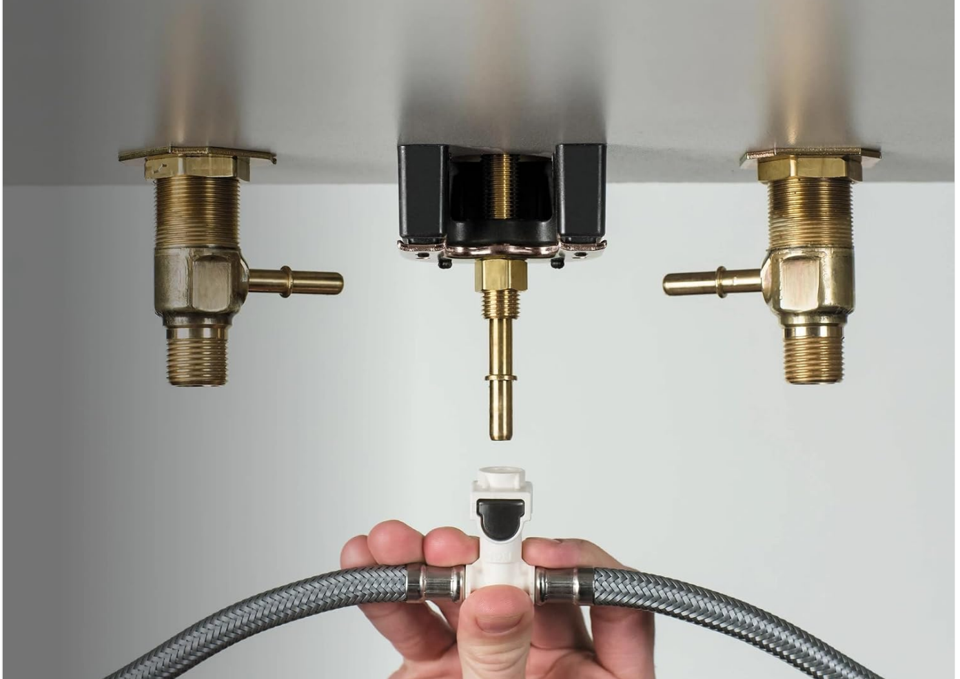
Figure 4: Illustration of the Duralock quick connect system, designed for easy and secure water line attachment.
