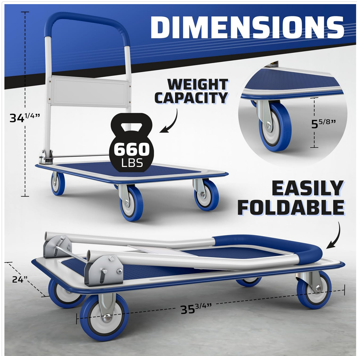
Figure 1: Dolly dimensions and folding mechanism. Note the 35-3/4" length, 24" width, and 34-1/4" height when unfolded. It folds to approximately 9-1/2" height for storage.
