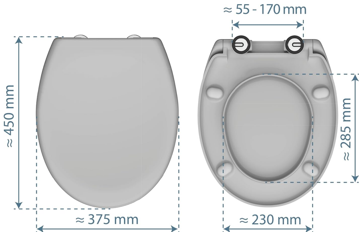
Image 4: Technical drawing showing the dimensions of the toilet seat. The overall length is approximately 450 mm, width 375 mm. The inner opening is approximately 285 mm long and 230 mm wide. The hinge distance is adjustable from approximately 55 mm to 170 mm.
