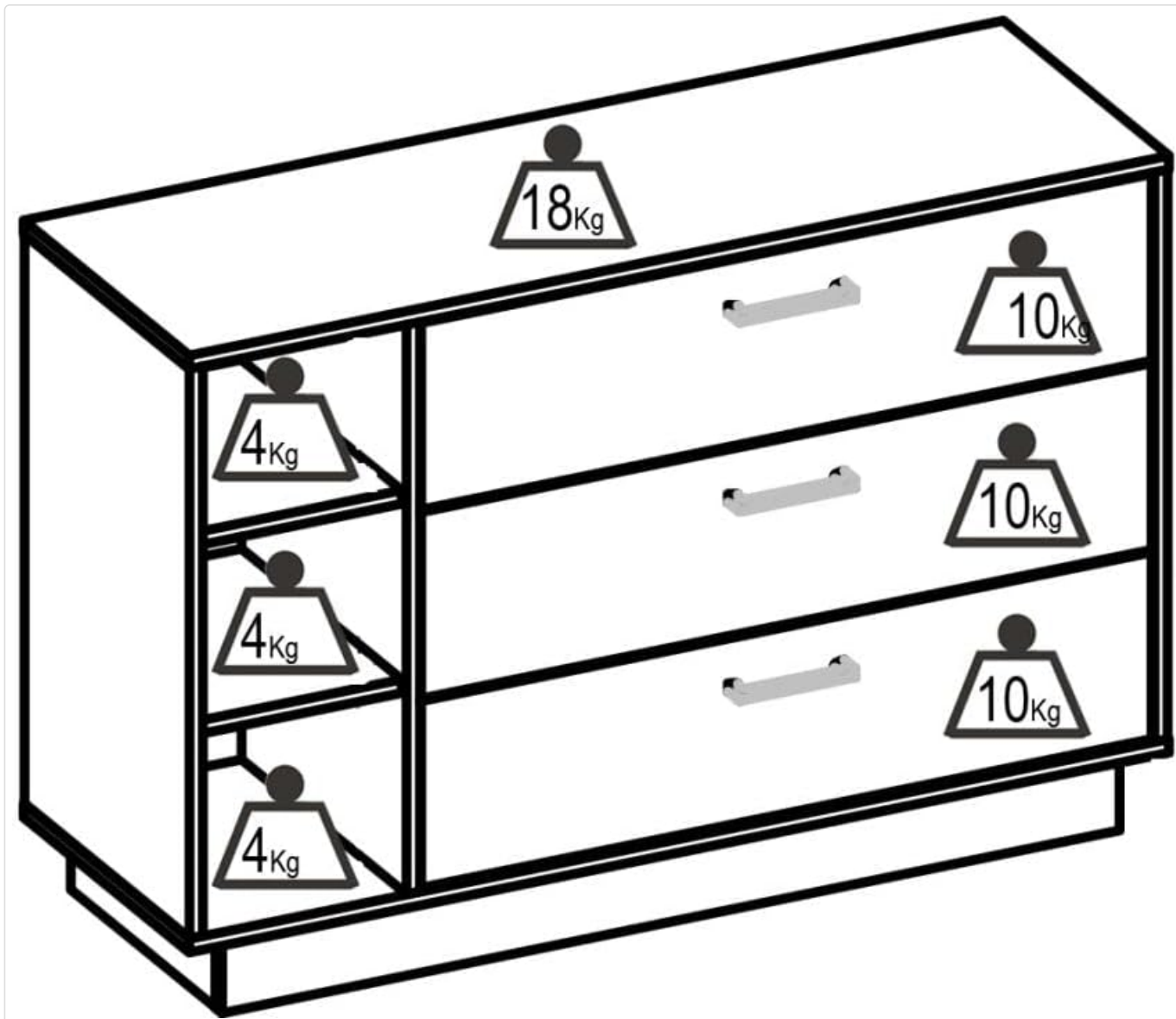
Figure 2: Diagram illustrating the maximum weight capacities for the Leandre chest of drawers: 18 kg on the top surface, 10 kg per drawer, and 4 kg per niche shelf.
