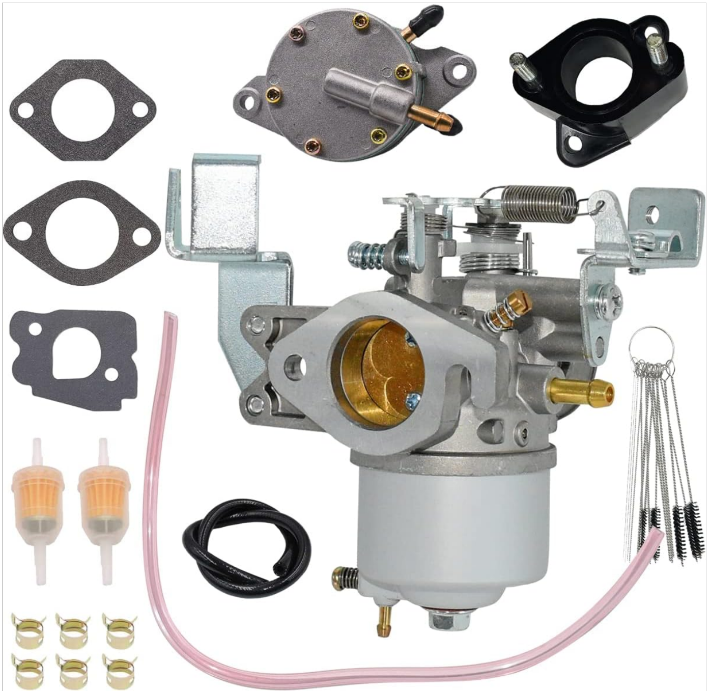
Figure 2: All components included in the JDLLONG J38-14101-02 Carburetor kit. This visual representation helps confirm the presence of all parts.
