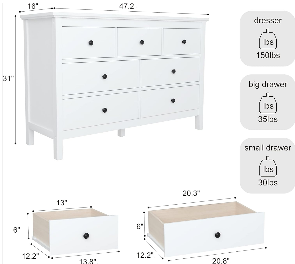
Image 3.1: Overall dimensions and drawer capacities of the dresser.
