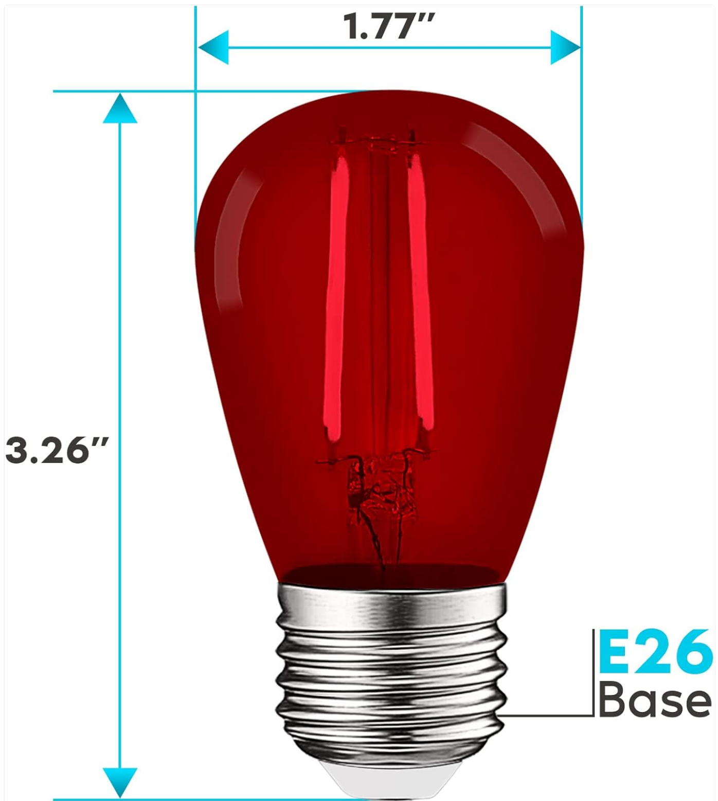
Image: Dimensions of the S14 Edison LED Red Light Bulb.
