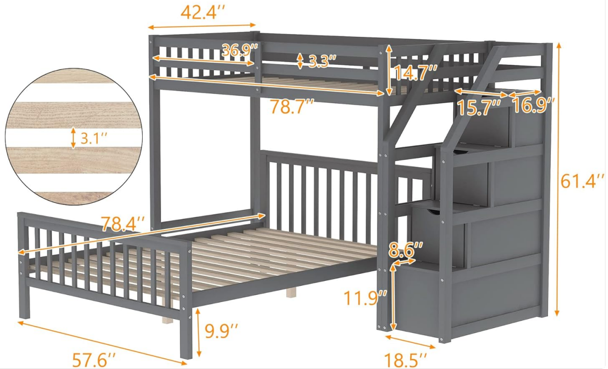
Image: Detailed dimensions of the bunk bed structure.
