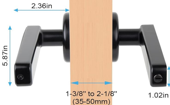
Figure 2: Door dimensions and latch adjustment.
