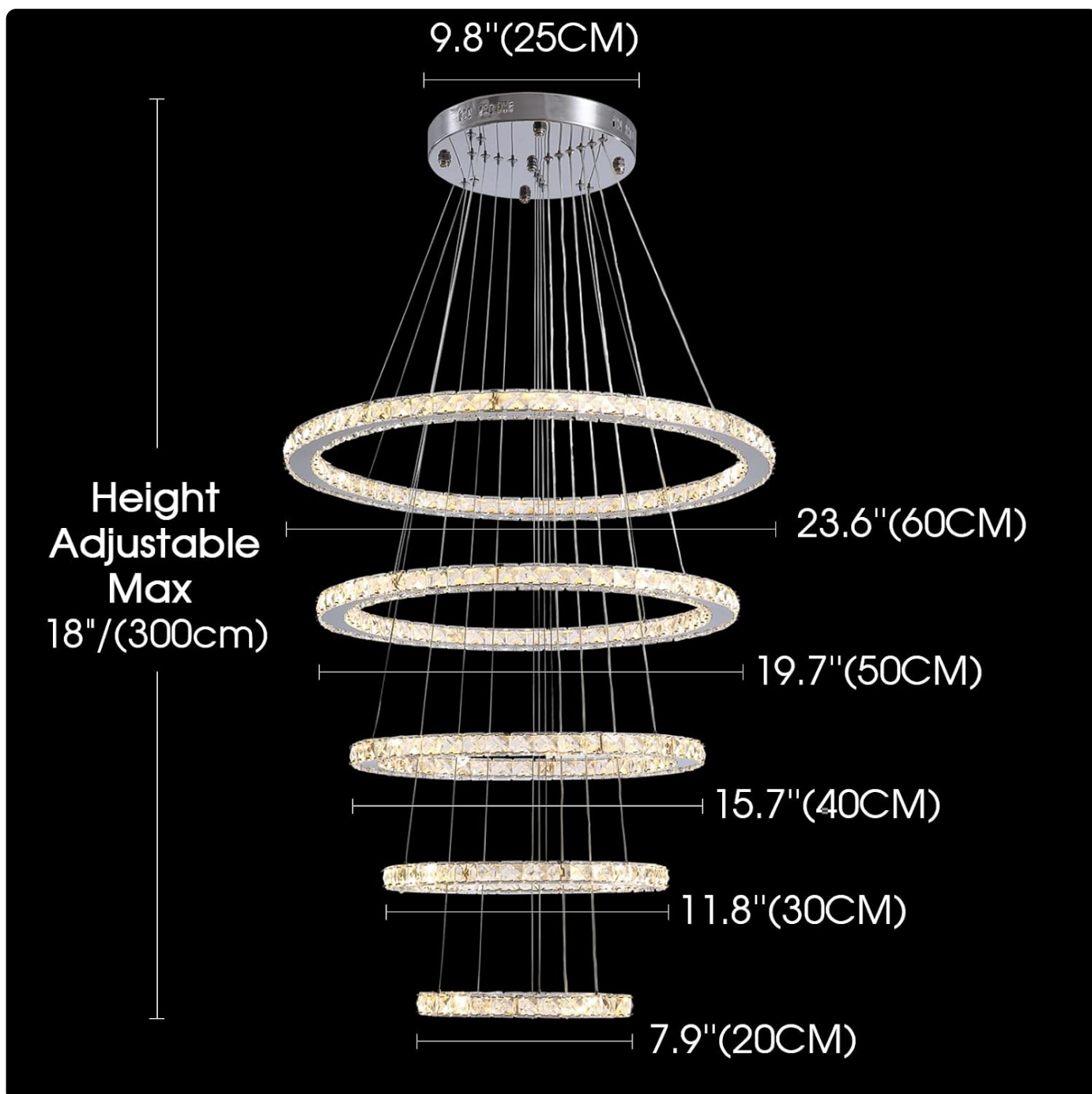
Figure 5: Chandelier dimensions and maximum adjustable cable length (118 inches / 300 cm).
