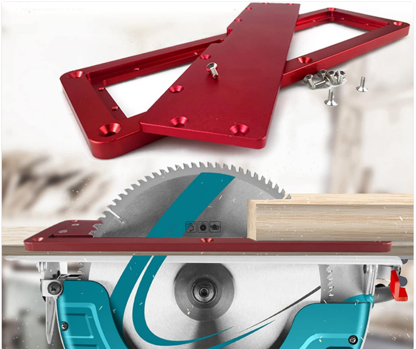
Figure 2: A circular saw positioned beneath the flip cover plate, demonstrating how the plate allows for cutting wood from an inverted saw setup. This illustrates the practical application of the product for woodworking tasks.
