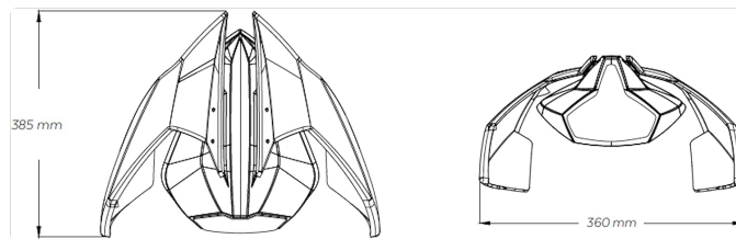
Figure 2: Technical drawing of the Puig Sport Screen, showing its overall shape and key dimensions (385 mm height, 360 mm width).
