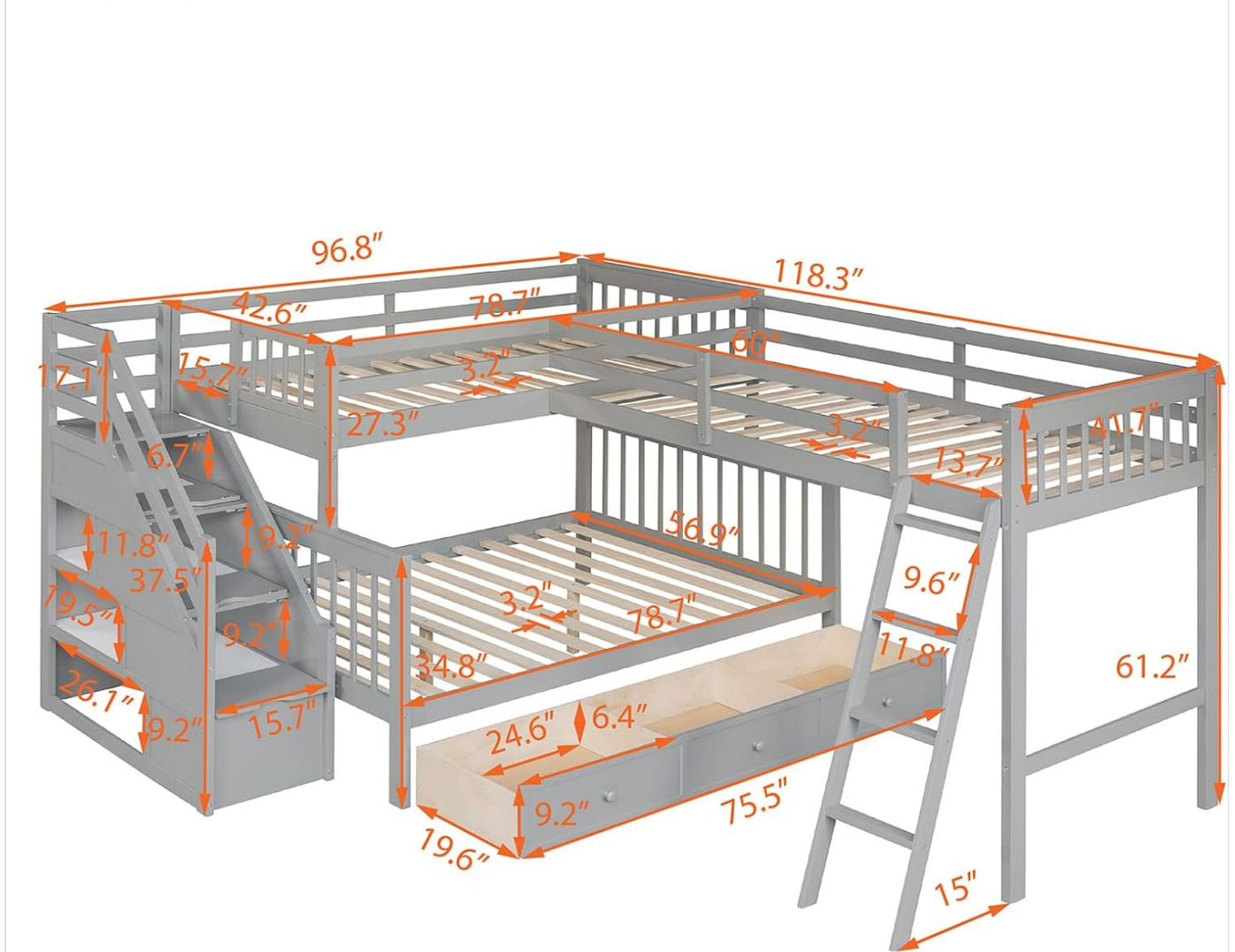
Image 8.1: A technical diagram illustrating the precise dimensions of the Bellemave L-Shape Triple Bunk Bed in inches.
