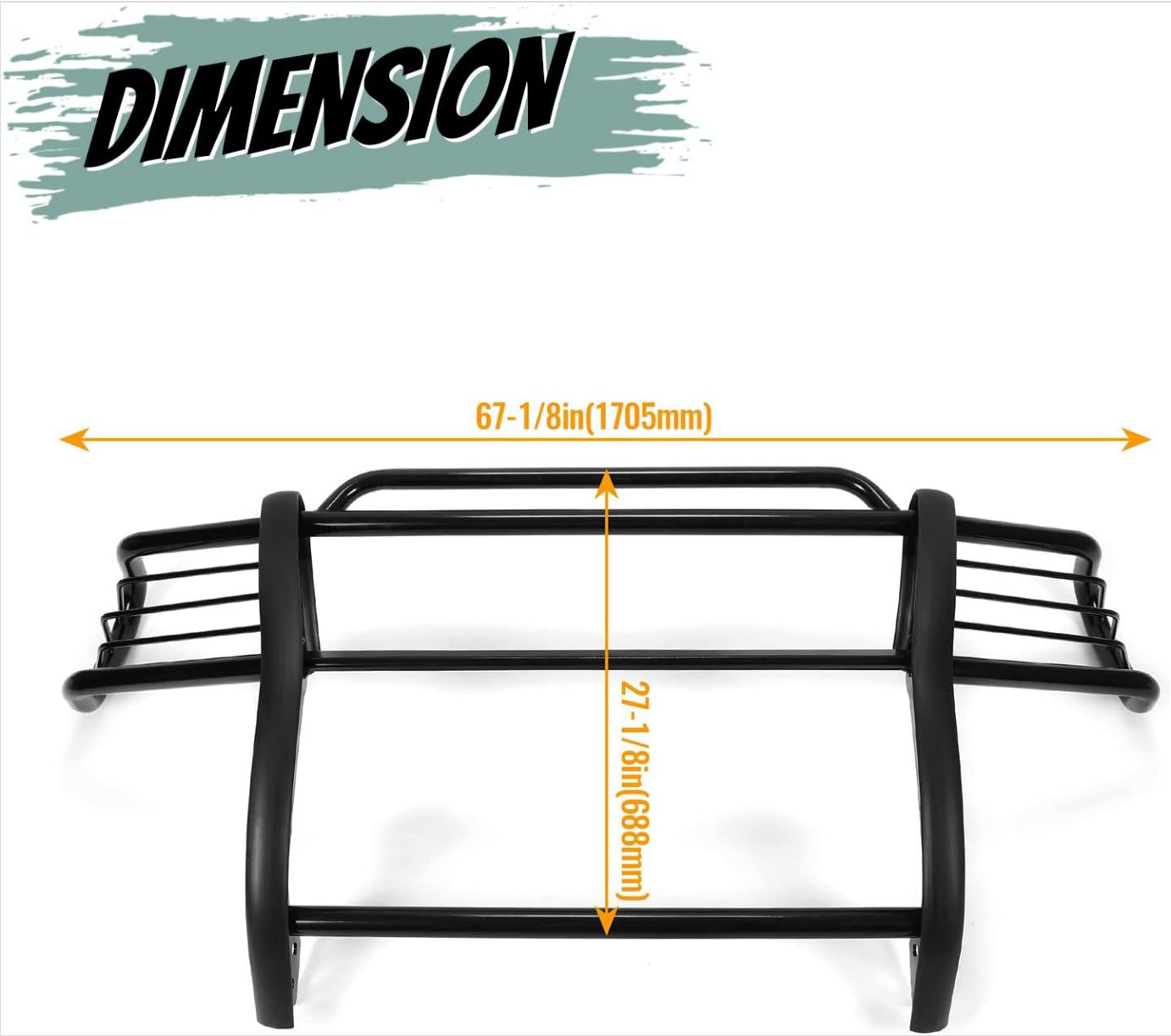
Image: A diagram illustrating the overall dimensions of the brush grille guard, including width and height.
