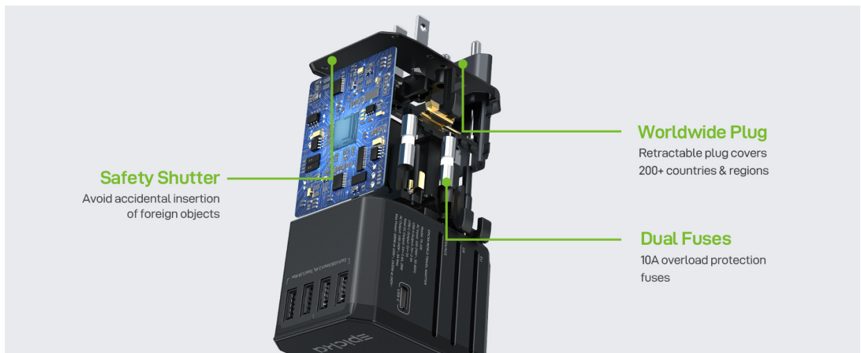
Image: An exploded view of the adapter highlighting its worldwide plug mechanism, safety shutters to prevent accidental insertion, and dual 10A overload protection fuses.
