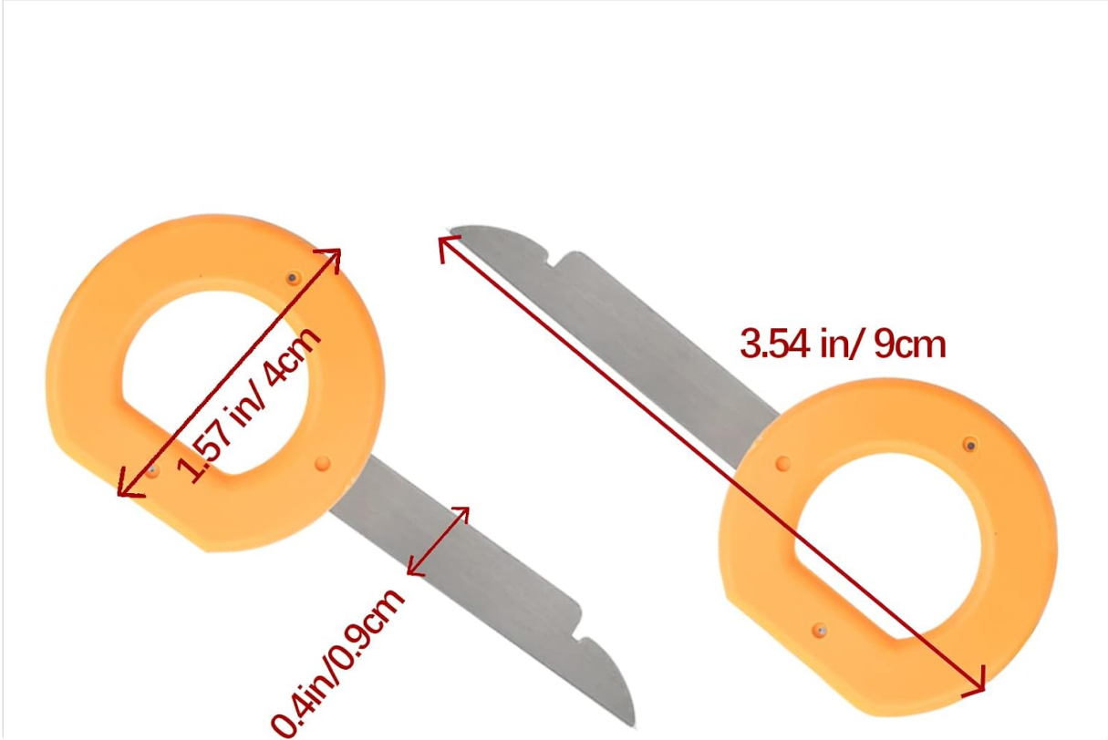
Image: Detailed diagram illustrating the specifications and dimensions of a single TEMI radio removal tool.
