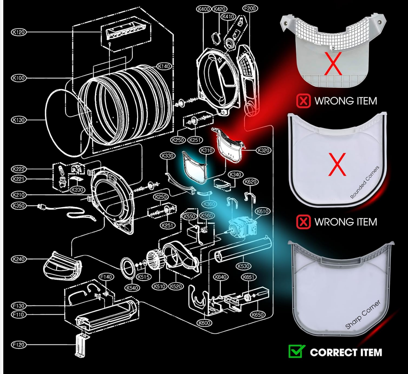
Image 4.2: Visual guide to help identify and order the correct lint filter shape for your dryer model.
