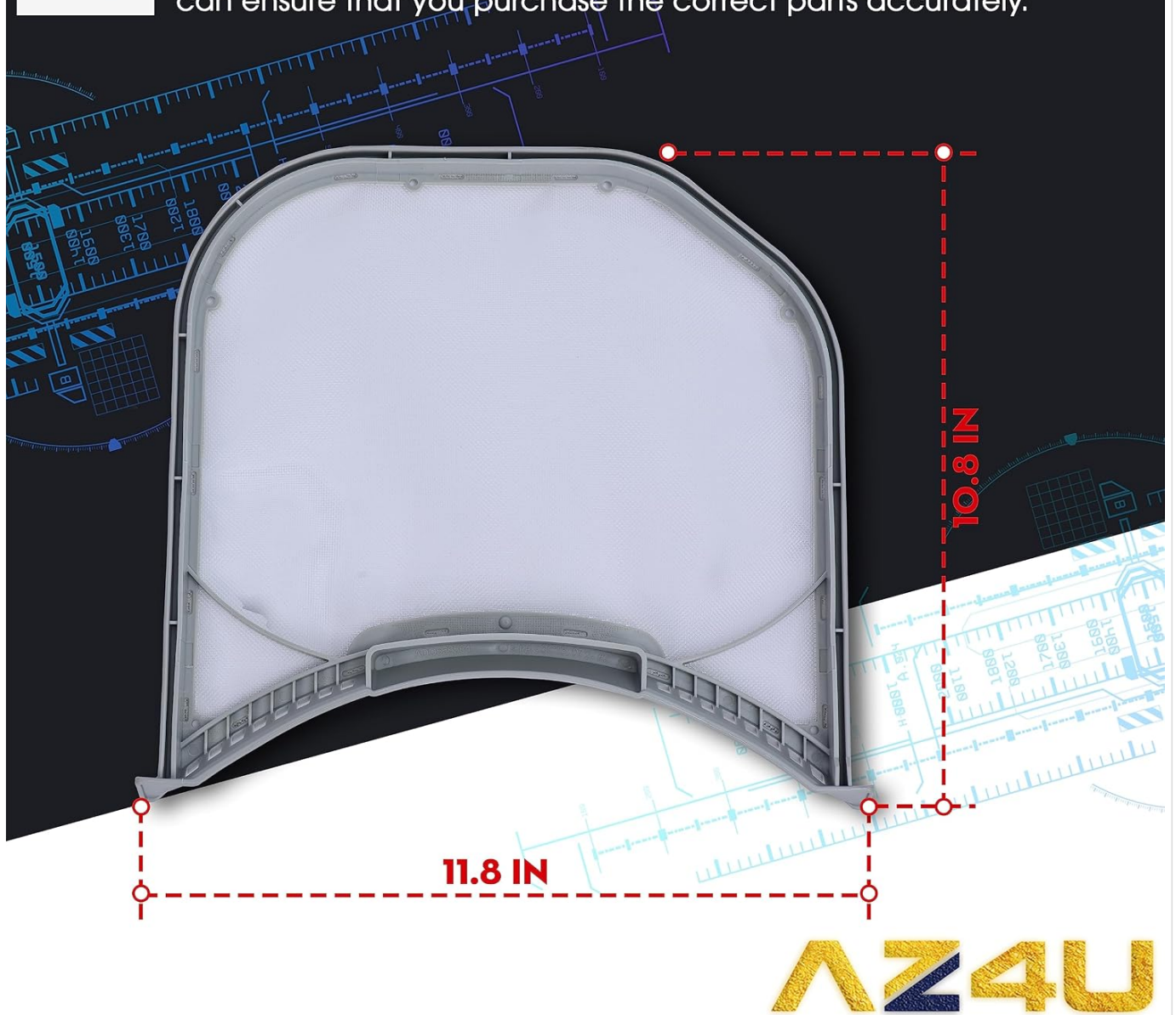
Image 5.1: Detailed dimensions of the lint filter for compatibility verification.
