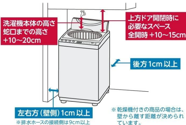
Figure 3.1: Detailed dimensions and required clearances for installation.
