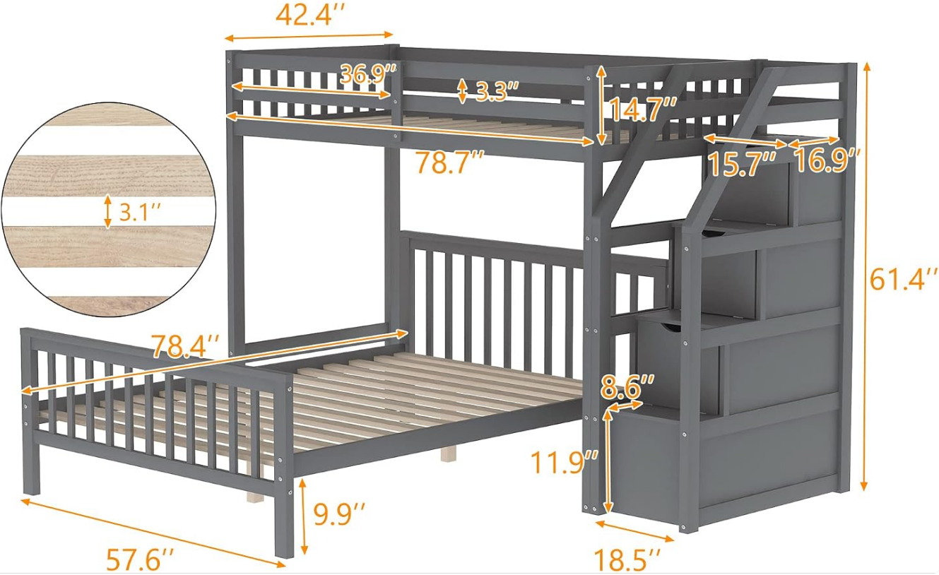
Image: Comprehensive diagram illustrating all key dimensions of the bunk bed and staircase unit in inches.
