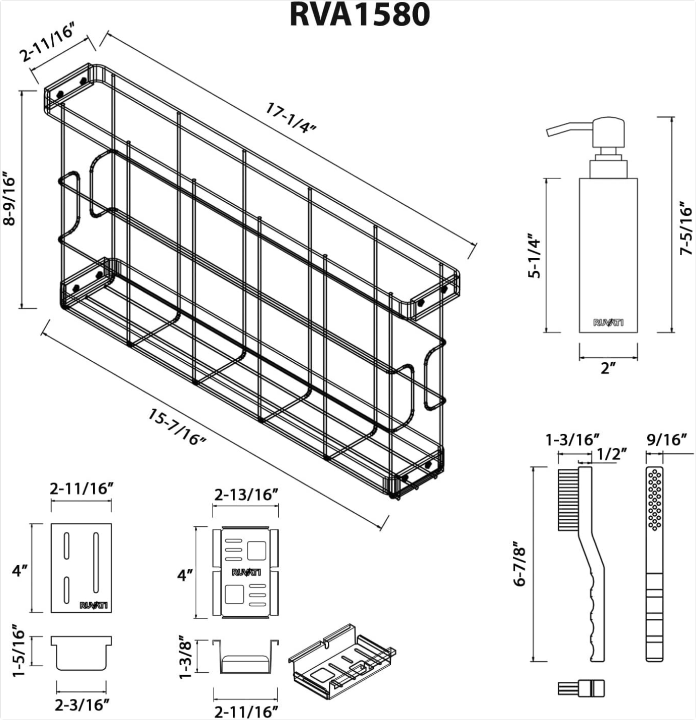
This detailed diagram provides precise measurements for the Ruvati RVA1580 Workstation Organizer caddy, including its overall dimensions and the sizes of the individual accessories like the soap dispenser, sponge tray, knife block, and cleaning brush.
