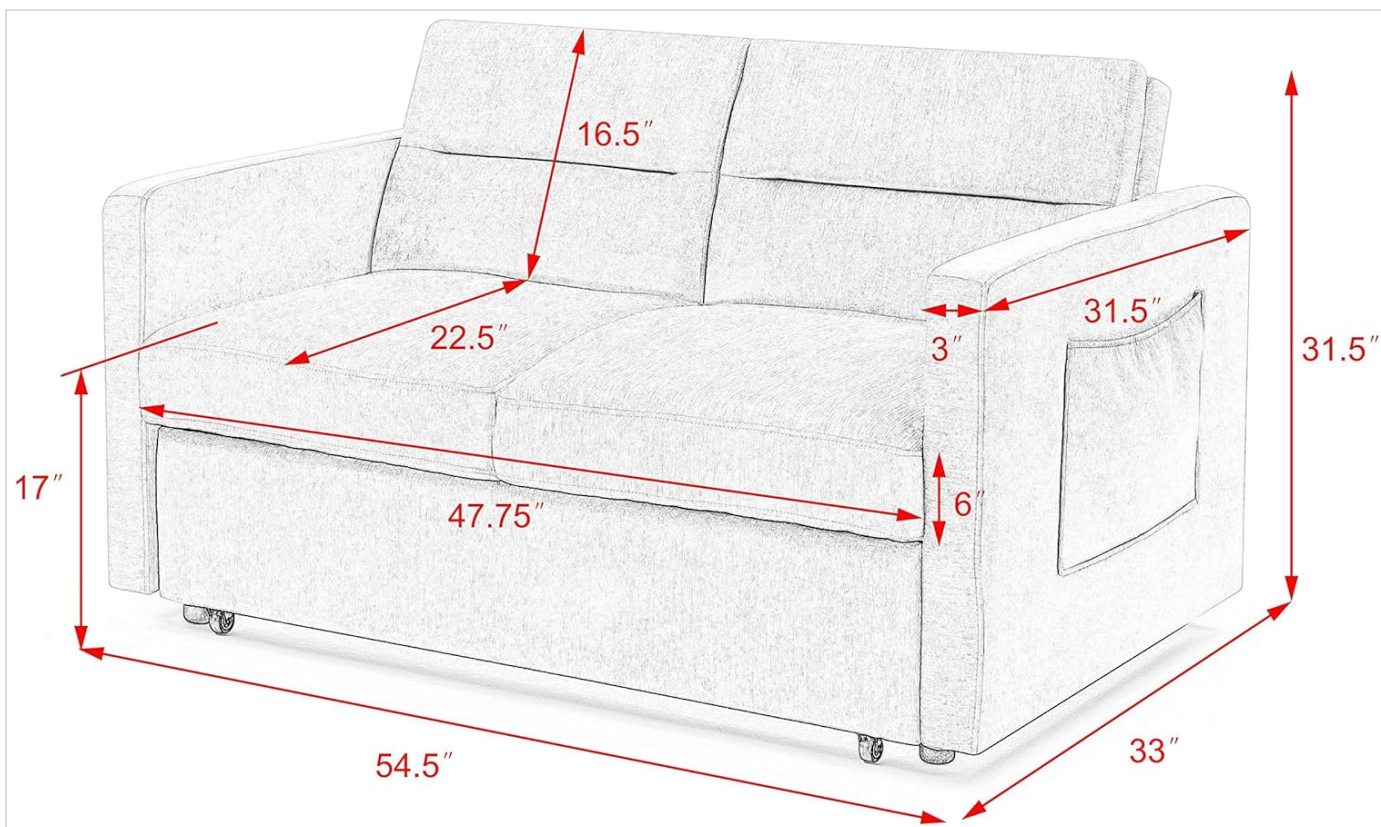
Image: Technical drawing illustrating the dimensions of the sofa in its compact loveseat form.
