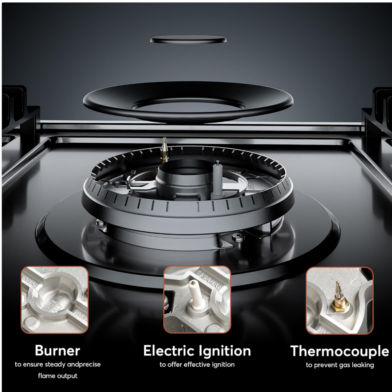
Image 3.3: Detailed view of a burner's internal components, highlighting the burner cap, electric ignition pin, and thermocouple for safety.
