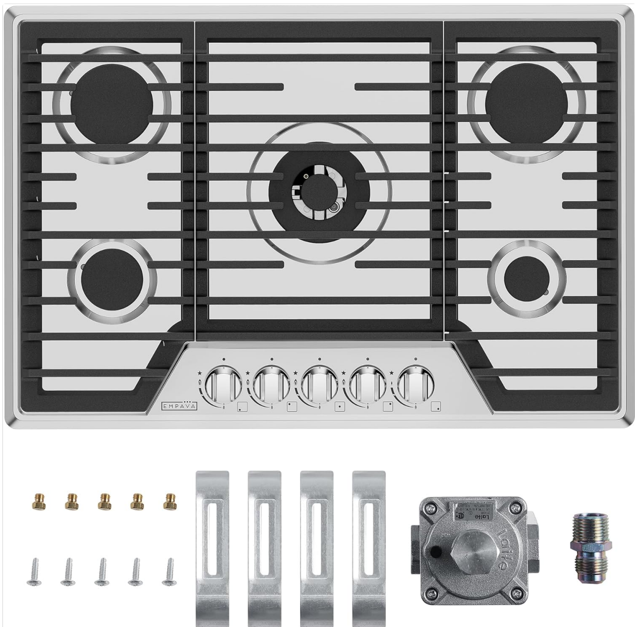
Image 4.2: Display of the various accessories provided for cooktop installation, such as gas nozzles, mounting hardware, and the gas pressure regulator.
