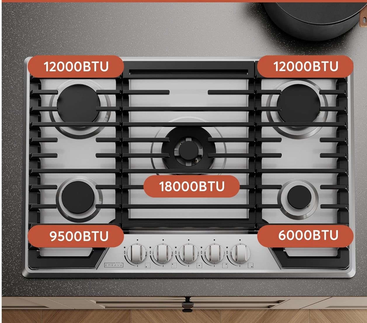
Image 3.2: Diagram illustrating the BTU output for each of the five burners on the cooktop, ranging from 6,000 BTU to 18,000 BTU.
