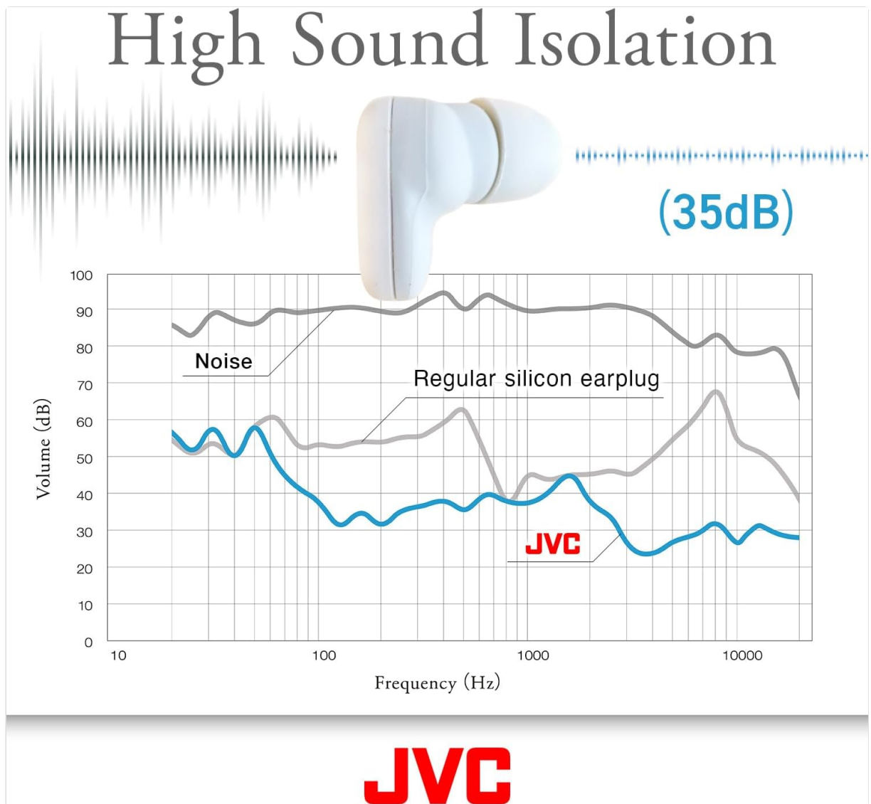
Image 3: A graph demonstrating the high sound isolation capability of JVC earplugs, showing a 35dB noise reduction across various frequencies compared to standard earplugs.
