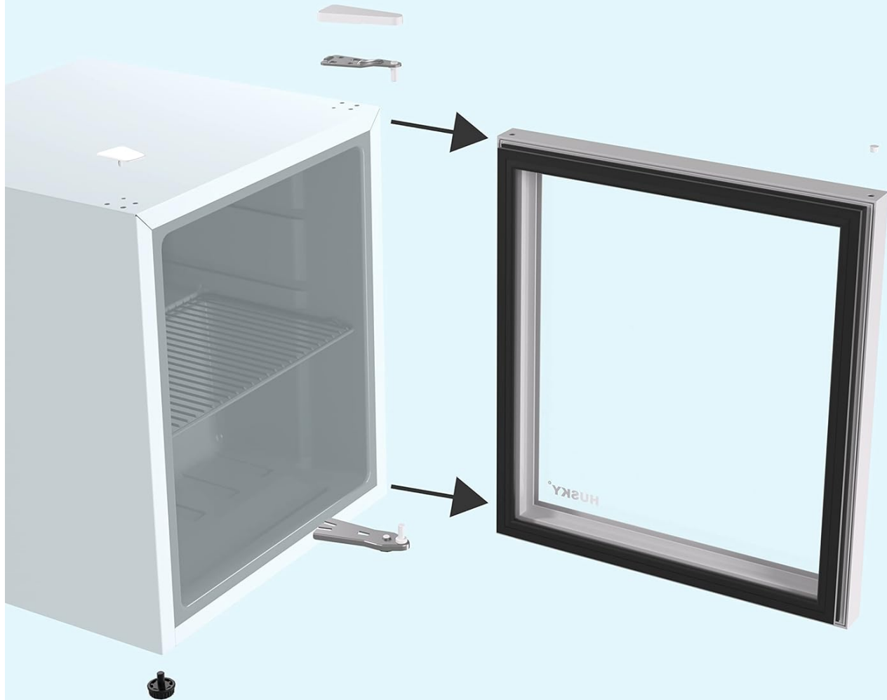
Diagram illustrating the process of reversing the door swing direction for flexible installation.
