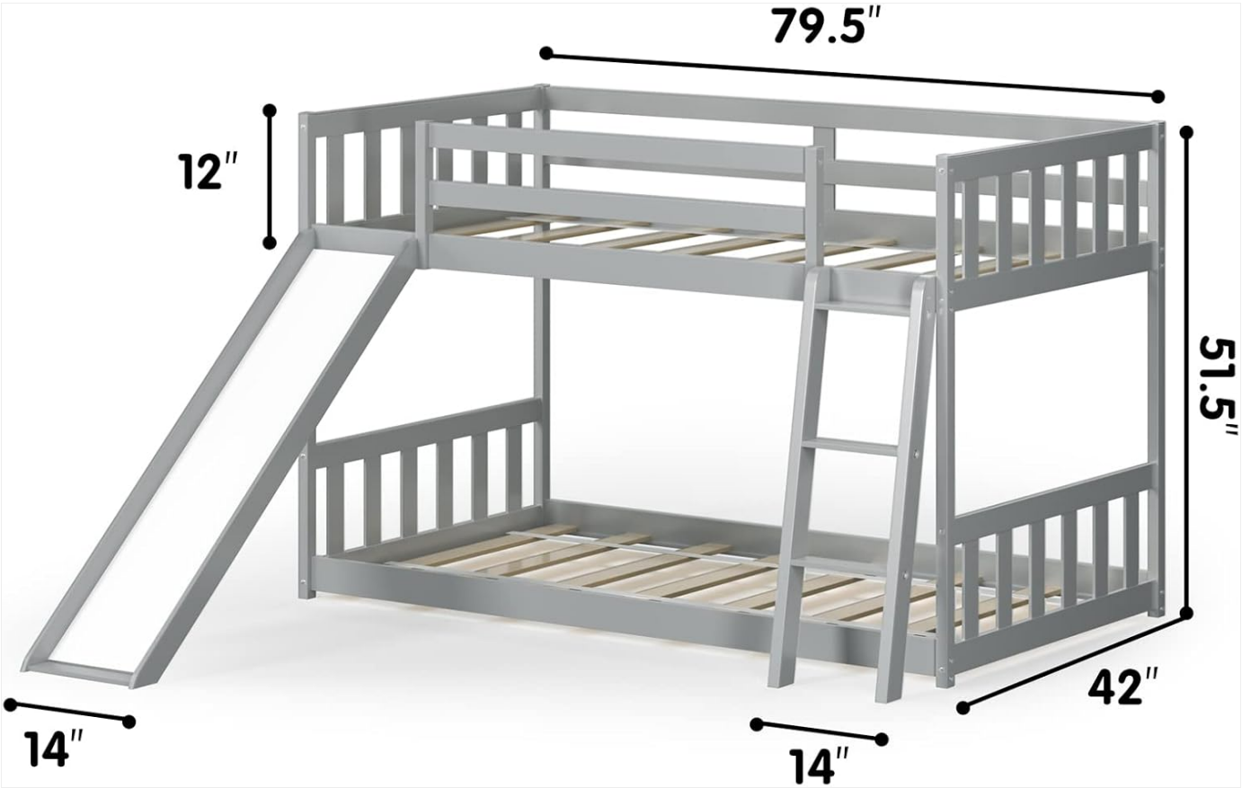
Figure 7.1: Dimensional diagram of the KOMFOTT Wood Bunk Bed.
