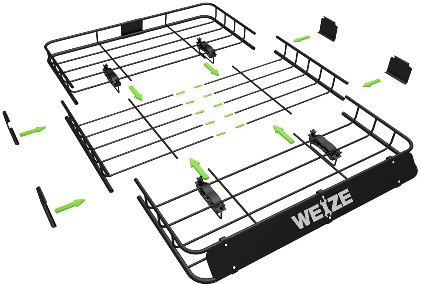
Figure 6.1: Assembly Diagram
