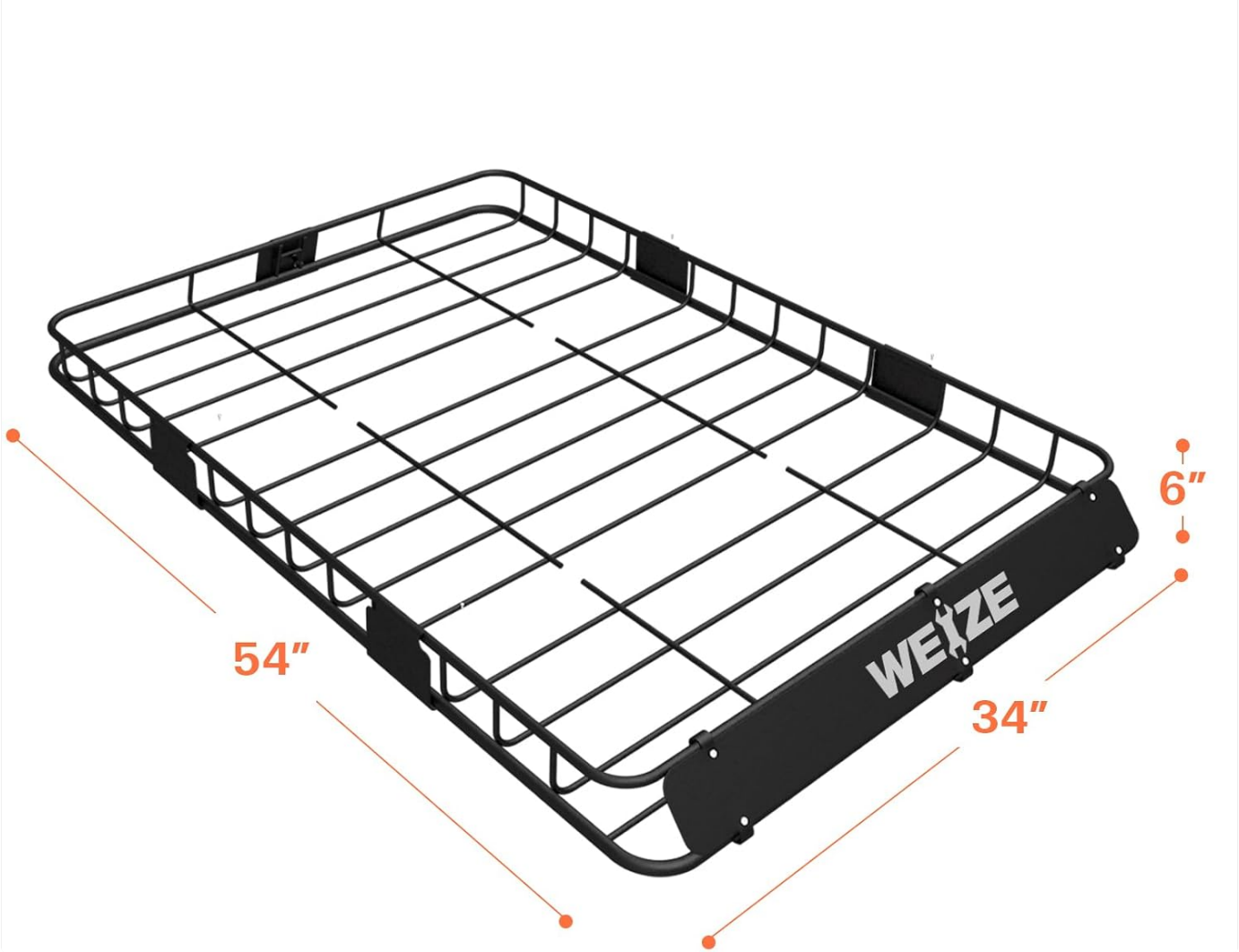
Figure 4.1: Product Dimensions
