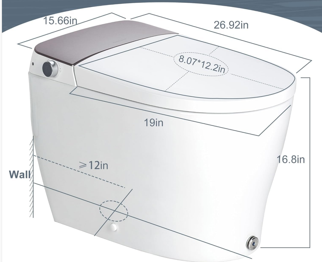
Image: Diagram showing the dimensions of the Casta Diva CD-Y060 Smart Toilet.
