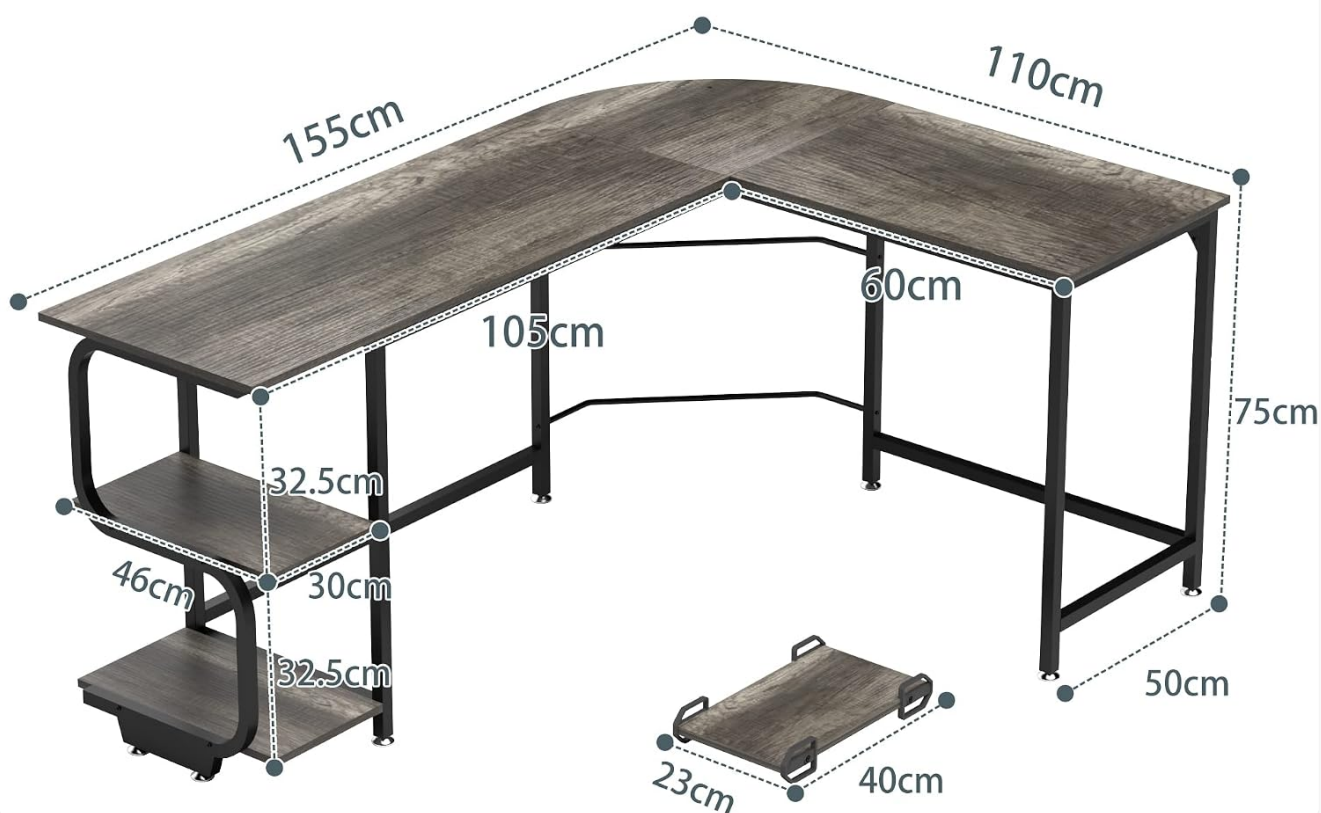
Image 3.1: Detailed dimensions of the Ulifance L-Shaped Computer Desk, including the main desktop and CPU stand measurements.
