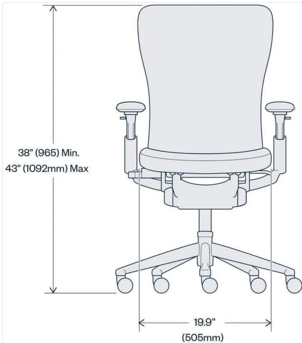
Figure 4: Front view dimensions.
