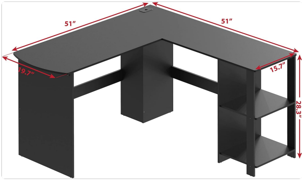
Figure 7.1: Detailed dimensions of the SHW L-Shaped Home Office Wood Corner Desk, showing 51" length on both sides, 19.7" depth, 15.7" shelf depth, and 28.3" height.
