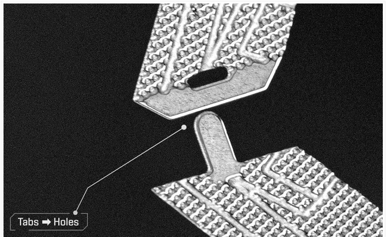
Image: A tab being bent to secure the connection between two metal pieces.
