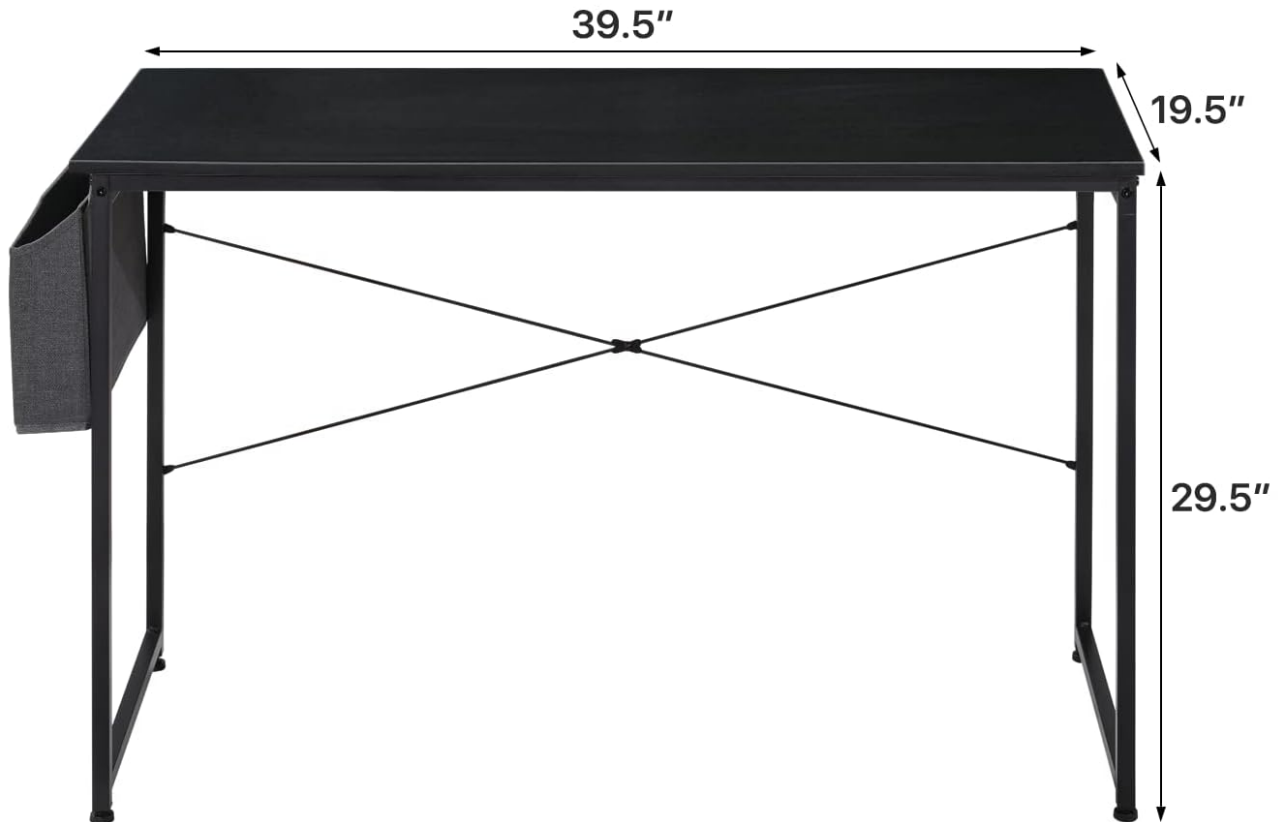
Figure 4.3: Overview of the desk structure, including the thickened metal frame.
