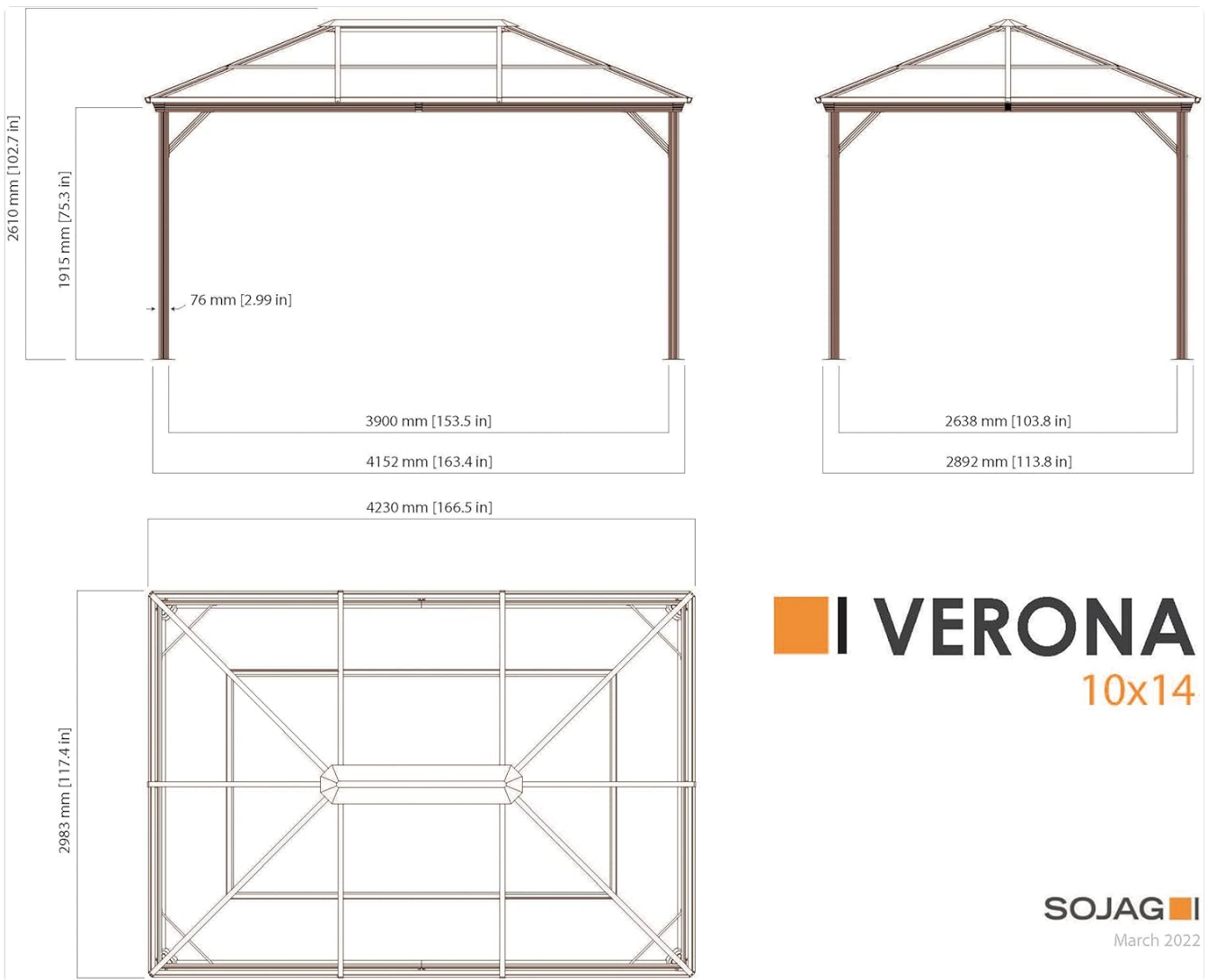
Image 7.1: Detailed technical drawing showing the dimensions of the Sojag Verona 10 Ft. X 14 Ft. Gazebo in both inches and millimeters.
