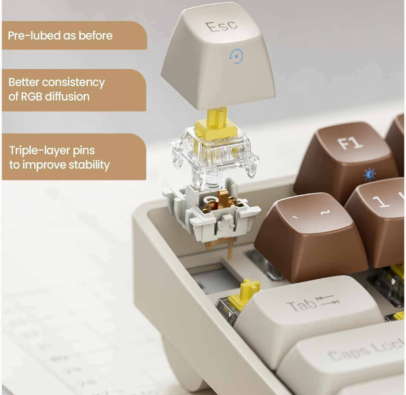
Image: An exploded view highlighting the components of the Gateron G Pro 3.0 Yellow switch, emphasizing its pre-lubricated design and improved lighting structure.
