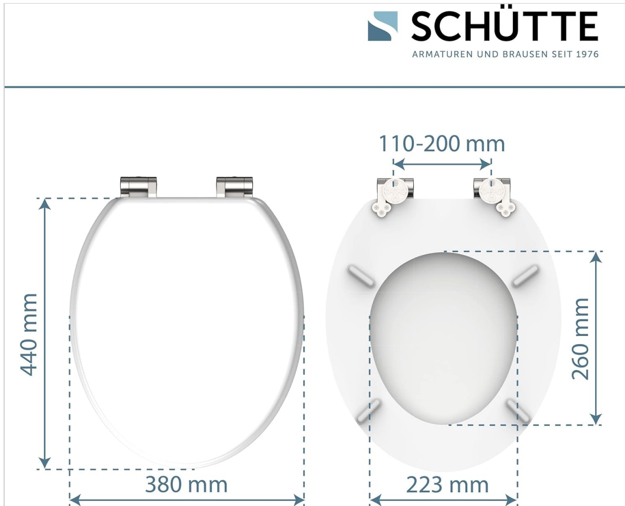
Image 2.1: Dimensional drawing of the Schütte 84100-A toilet seat, indicating key measurements for compatibility and installation, including hinge spacing (110-200 mm), seat width (380 mm), and length (440 mm).
