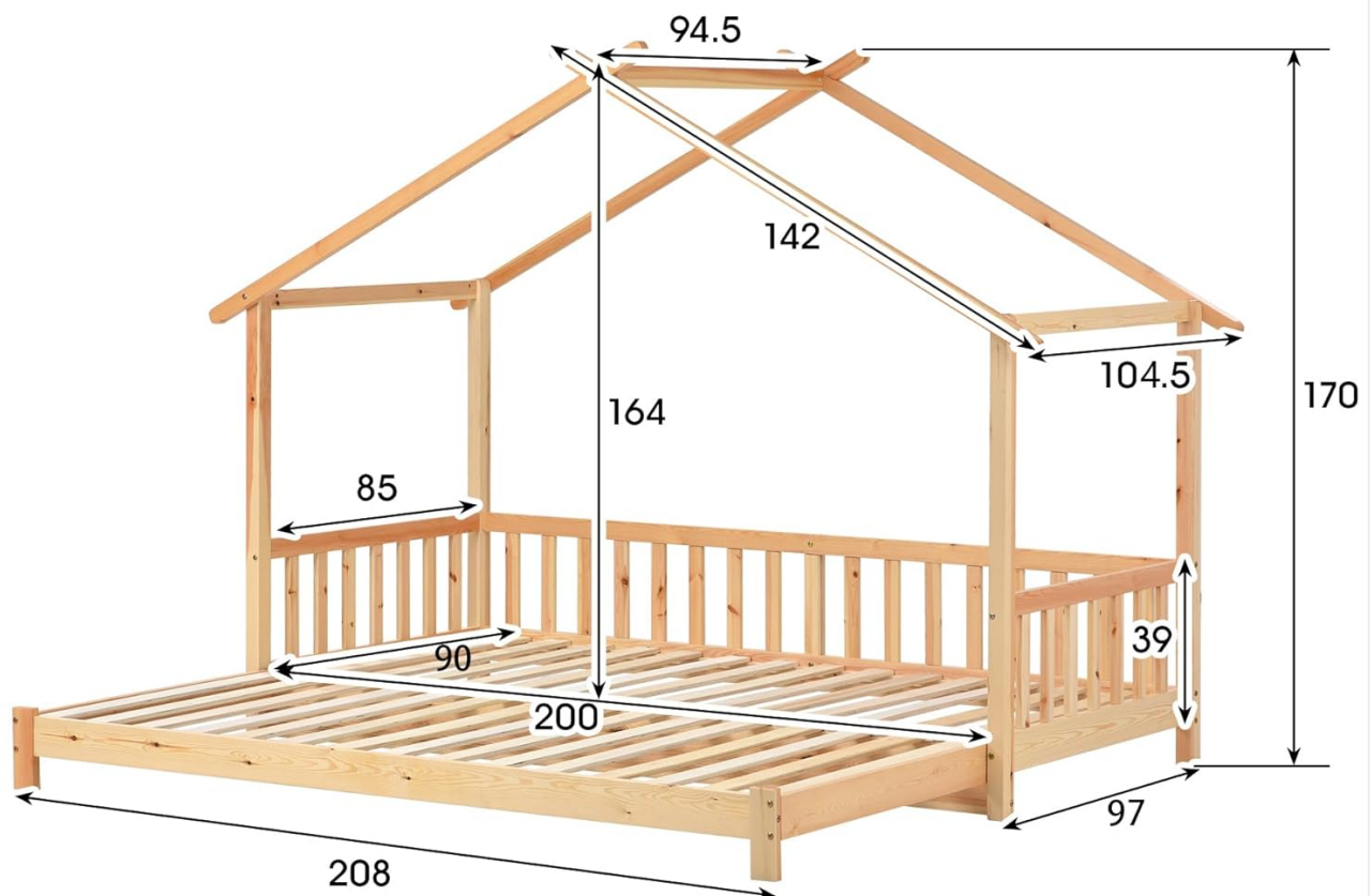
Figure 3.1: Detailed dimensions of the Merax House Bed, showing overall length (208 cm), width (97 cm / 182 cm when extended), and height (170 cm).
