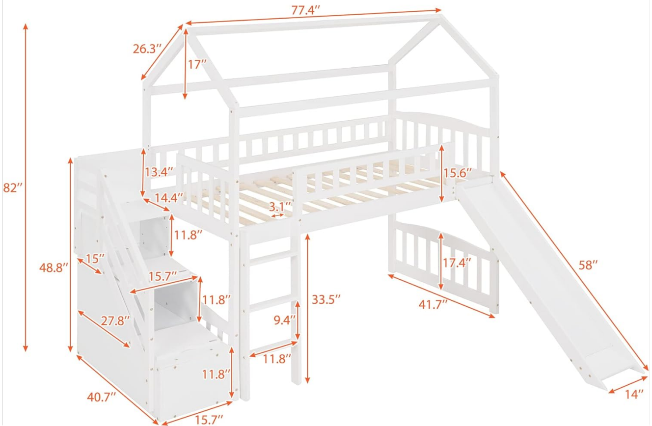
Image 2.1: Dimensional diagram of the loft bed, showing key measurements for planning and assembly.
